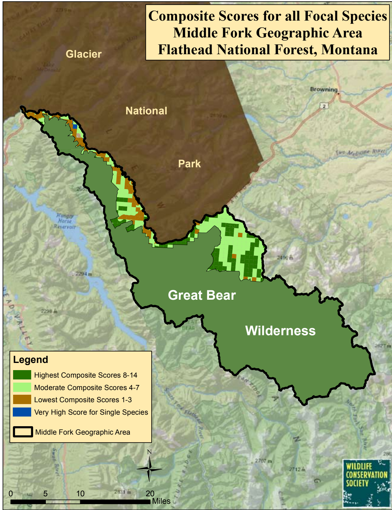
Figure 25. Distribution of composite scores for all focal species, Middle Fork Geographic Area, Flathead National Forest, Montana.
